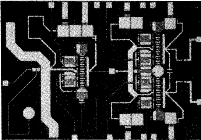
Figure 8: X-band Variable Power Amplifier (XVPA)
