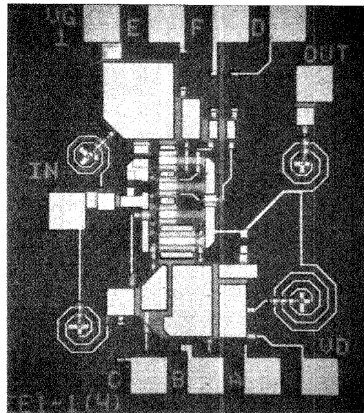
Figure 6: X/K u -band Variable Gain Amplifier
