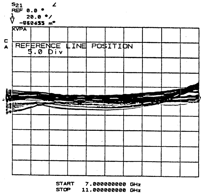
Figure 10: XVPA Incidental Phase Shift Across 64 States
